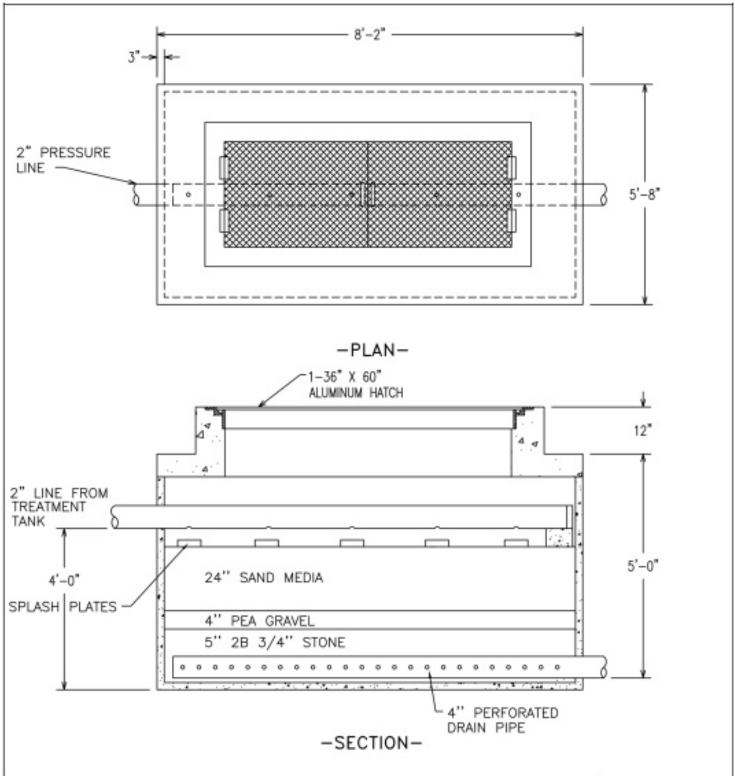
FREE ACCESS SAND FILTER 40 SQUARE FEET W/ ALUM. ACCESS DOOR
