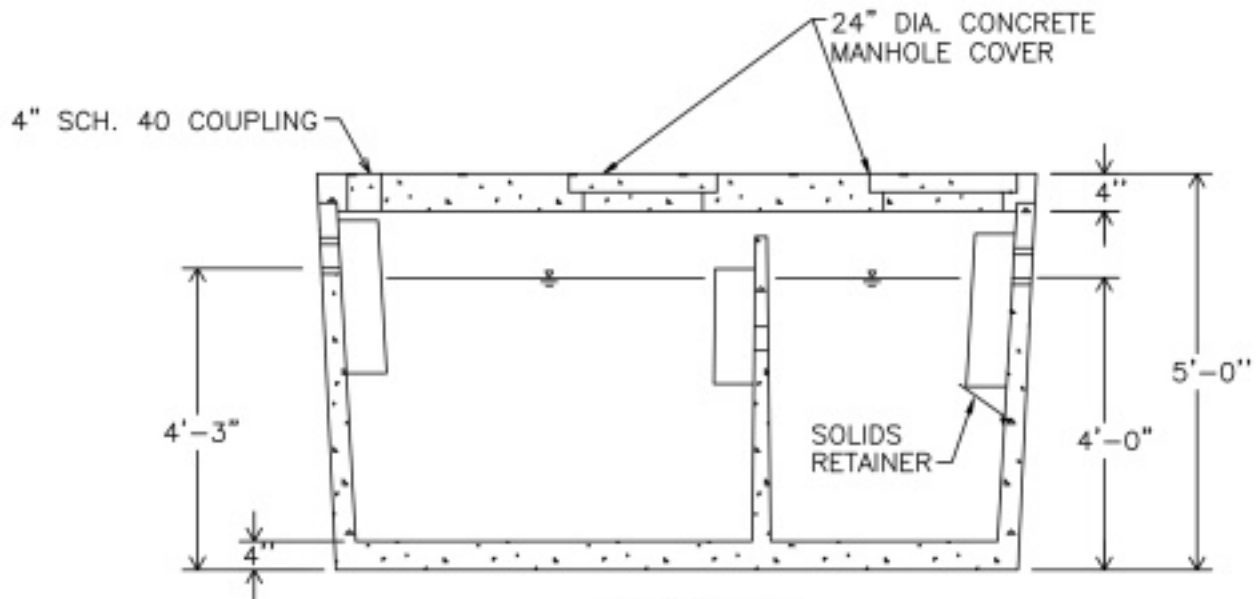
-SECTION-
