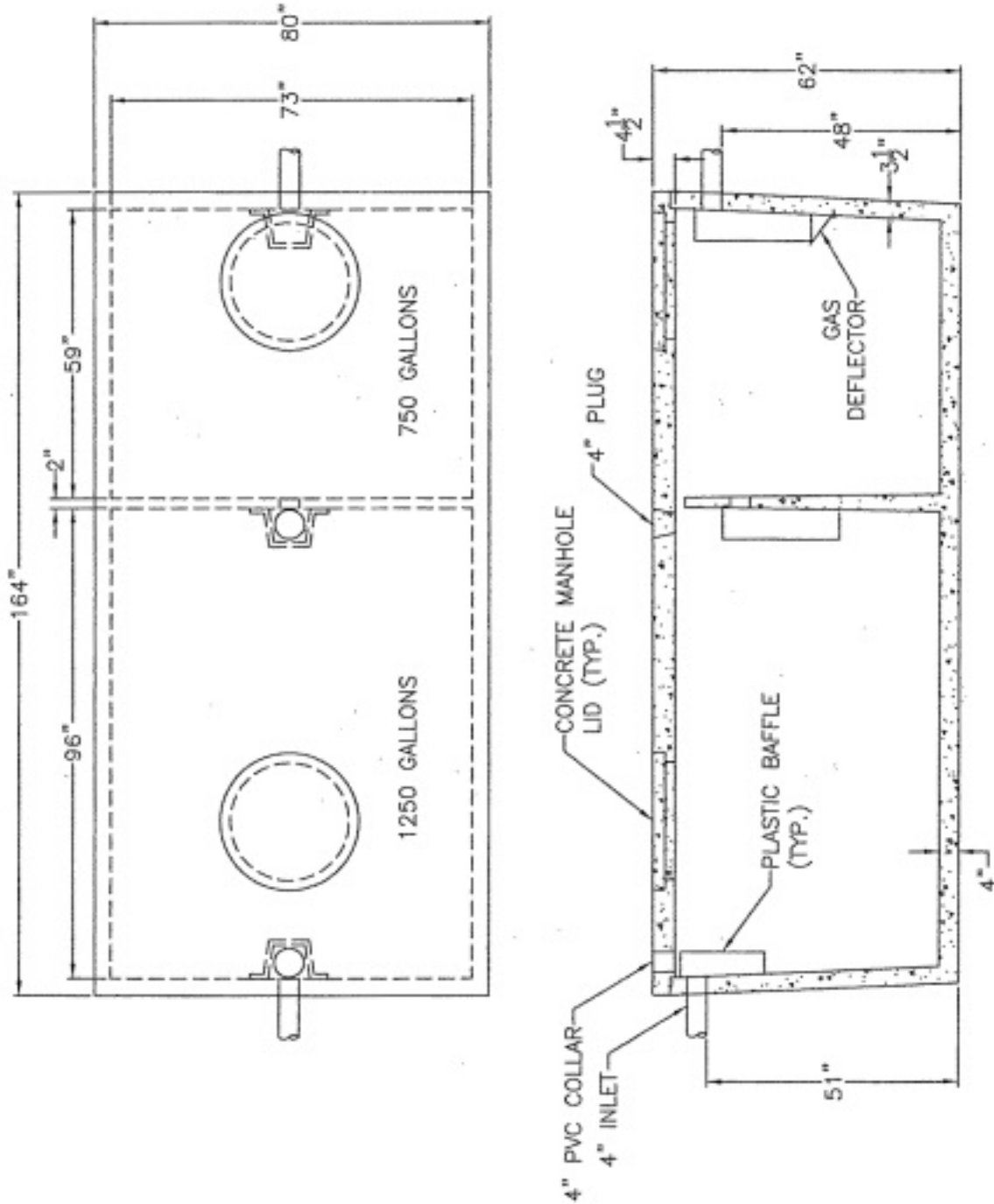
PRECAST 2 COMPARTMENT SEPTIC TANK 2000 GALLON CAPACITY
