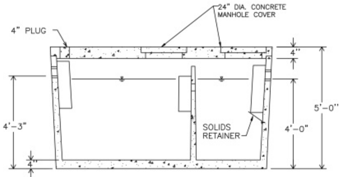
-SECTION-
